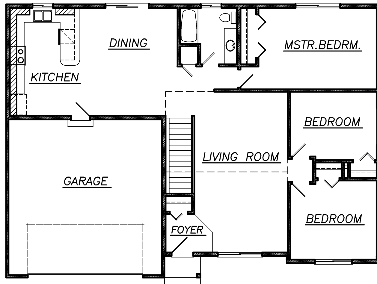
MAIN LEVEL 1421 SQ.FT.
