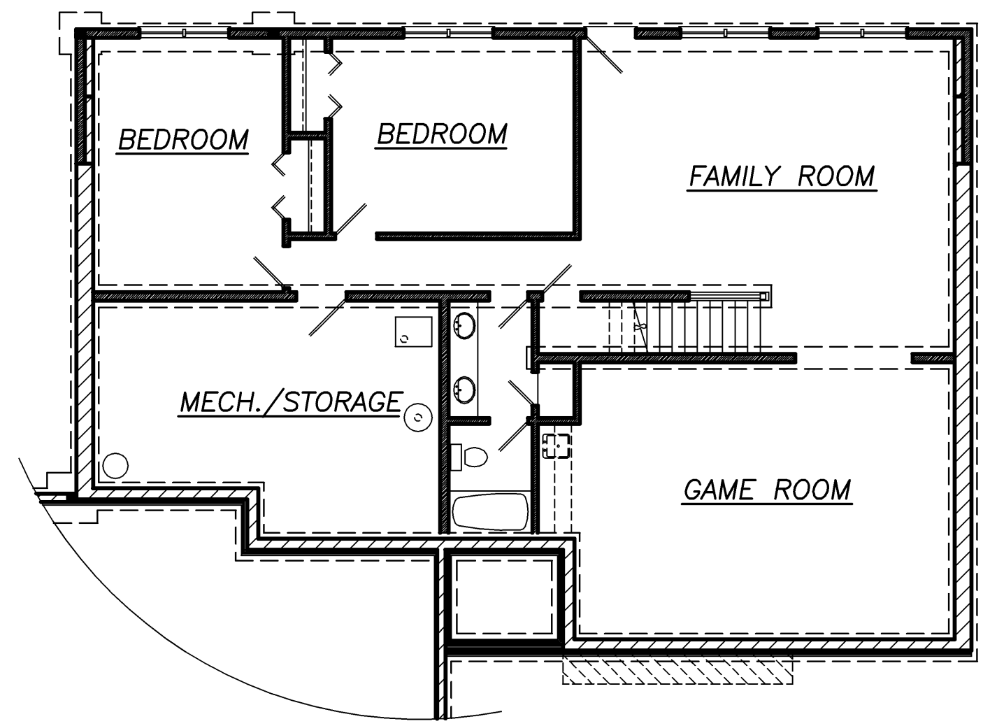
FOUNDATION PLAN 1374 SQ.FT. FINISHED
