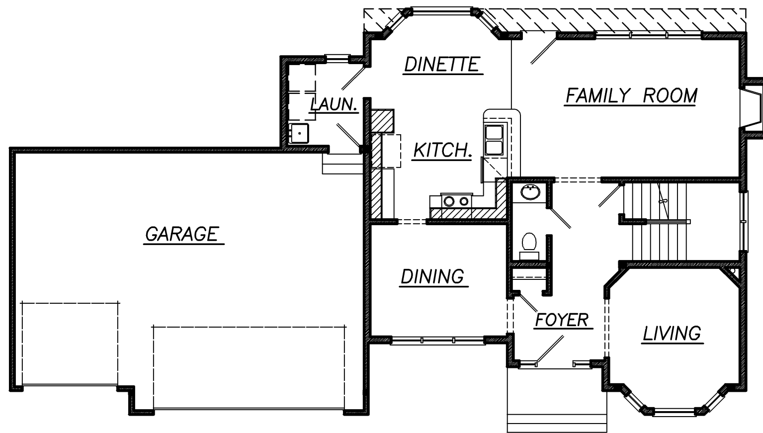
MAIN LEVEL 965 SQ.FT.
