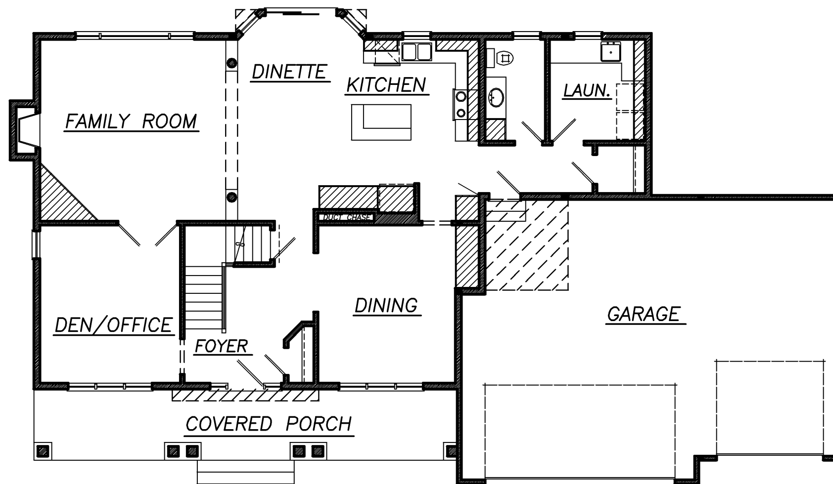
MAIN LEVEL 1347 SQ.FT.
