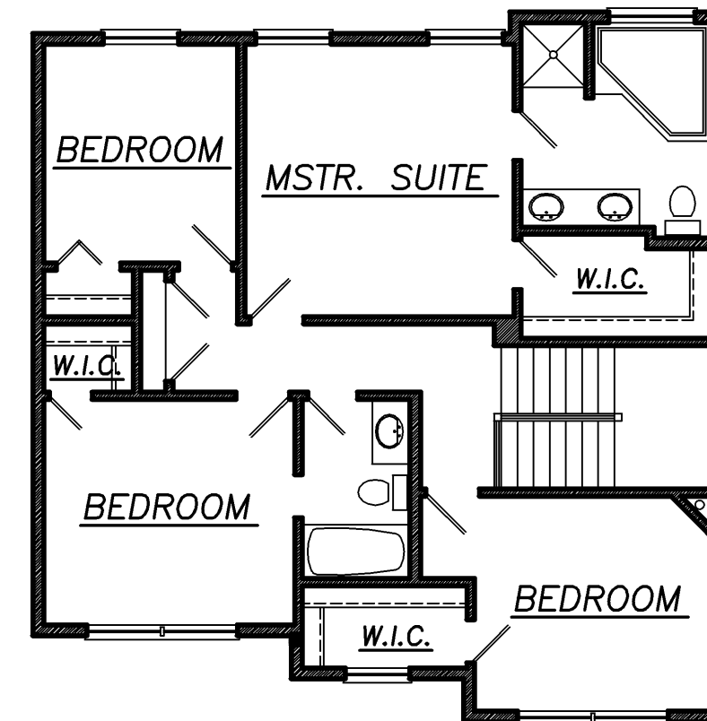
SECOND FLOOR 905 SQ.FT.
