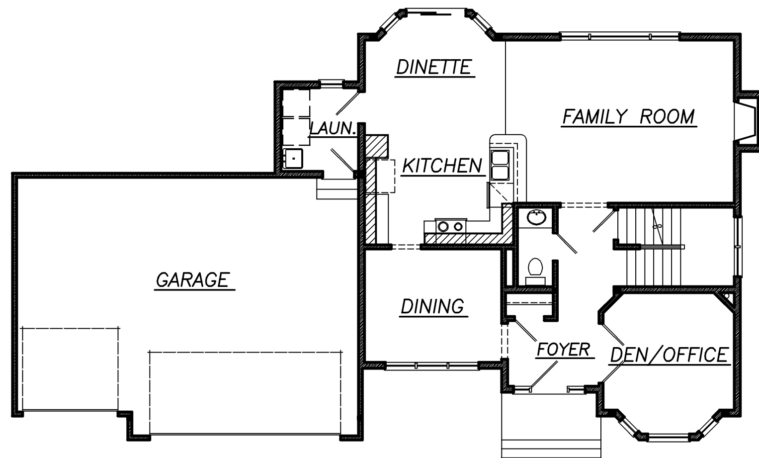
FIRST FLOOR 1046 SQ.FT.
