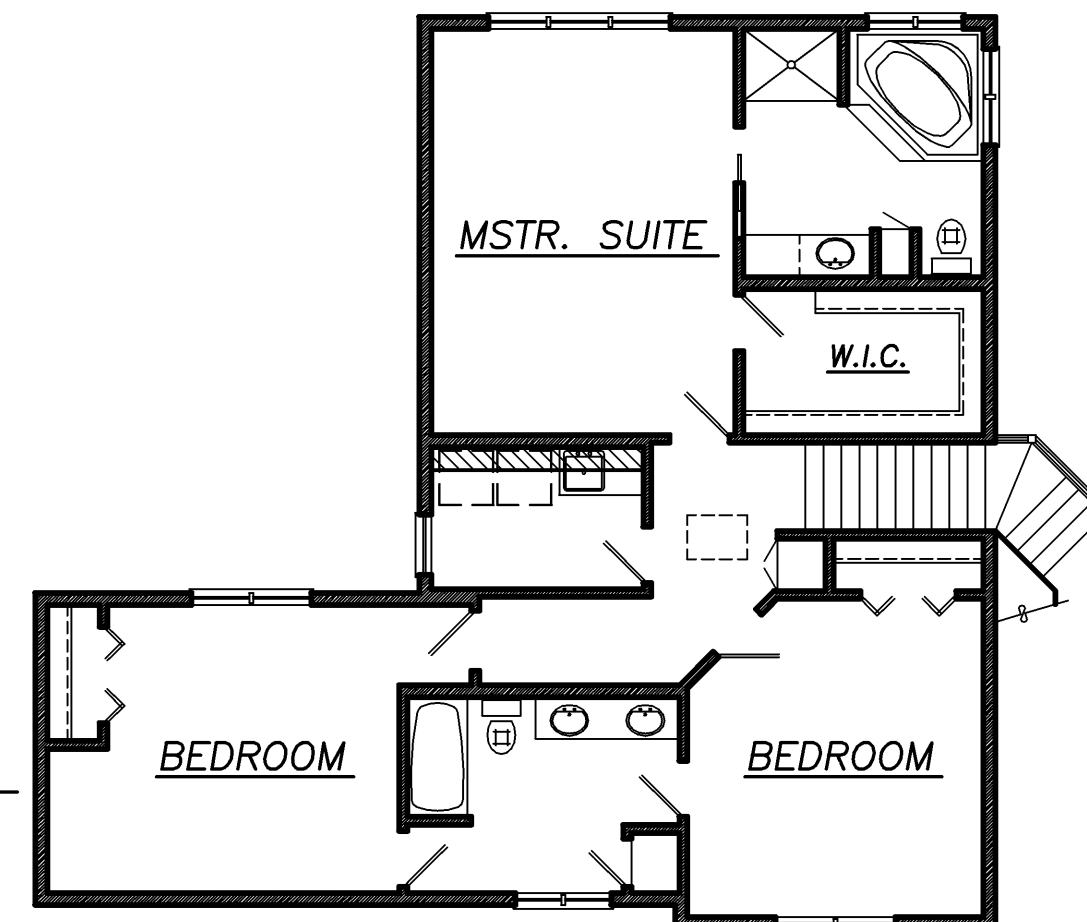
UPPER LEVEL 1109 SQ.FT.
